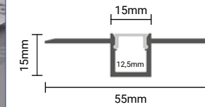
SKU: 5162 Silver Body- White Cover (L=2m) ■□
