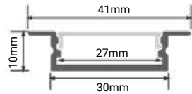
SKU: 5118 Silver Body- White Cover (L=2m) □□
