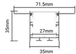
SKU: 5124 Silver Body- White Cover (L=2m) □□
