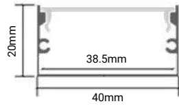
SKU: 5121 Silver Body- White Cover (L=2m) □□
